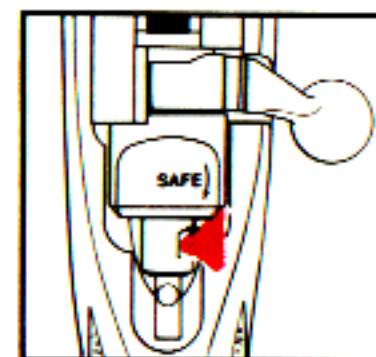
Figure 4. Safety selector in "SAFE" position. The selector is at its full rearward position and the tongue portion of the safety selector is fully nested in the groove in the cocking piece. When the safety selector is in this position, the bolt handle cannot be raised. The curved arrow on the bolt sleeve indicates the direction and motion of the safety selector to bring it to the "SAFE" position.
