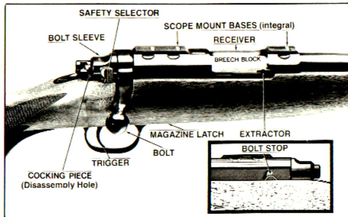
Figure 1. Components frequently referred to are identified. In this illustration the cocking piece is shown cocked (protruding from the rear of the bolt sleeve) revealing the disassembly hole in the lower portion of the cocking piece. The bolt stop (on the left side of the receiver) permits the bolt to be withdrawn simply by pressing down lightly with the thumbnail. The safety selector (shown in the "Fire" position) should be in the "Load-Unload" position when the bolt is being removed or being installed.
